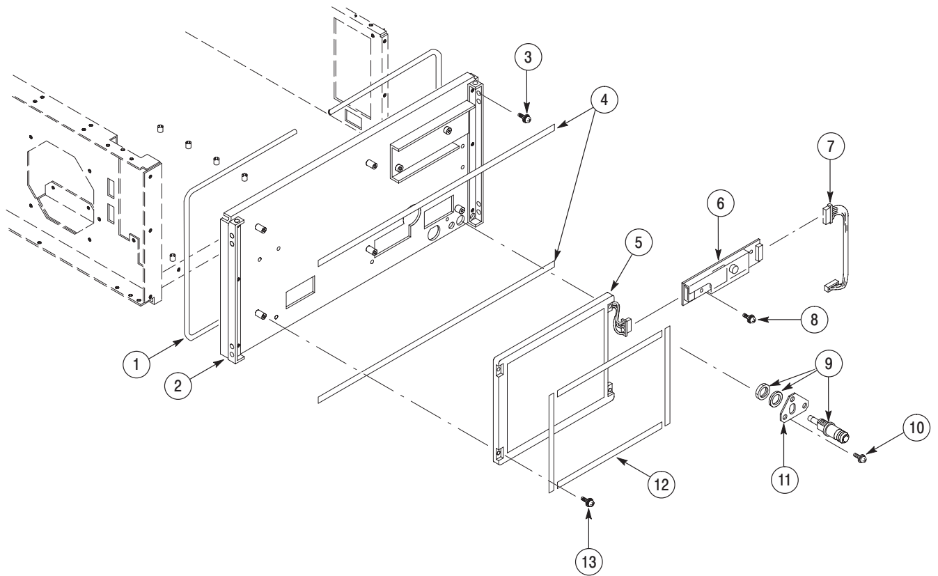
Figure 10-3: Front-panel assembly - 2
