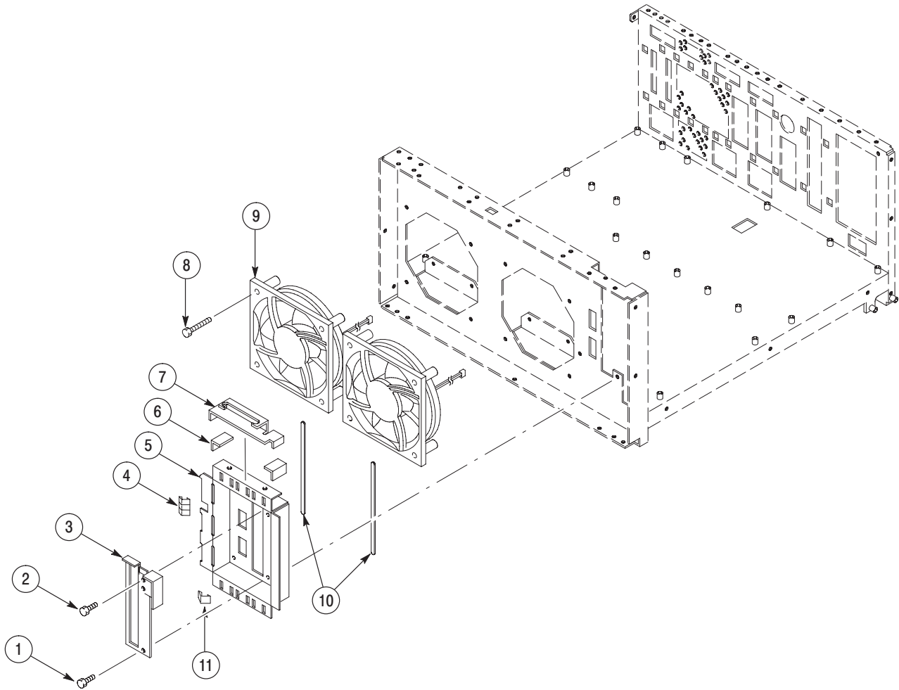
Figure 10-13: Chassis modules - 2
