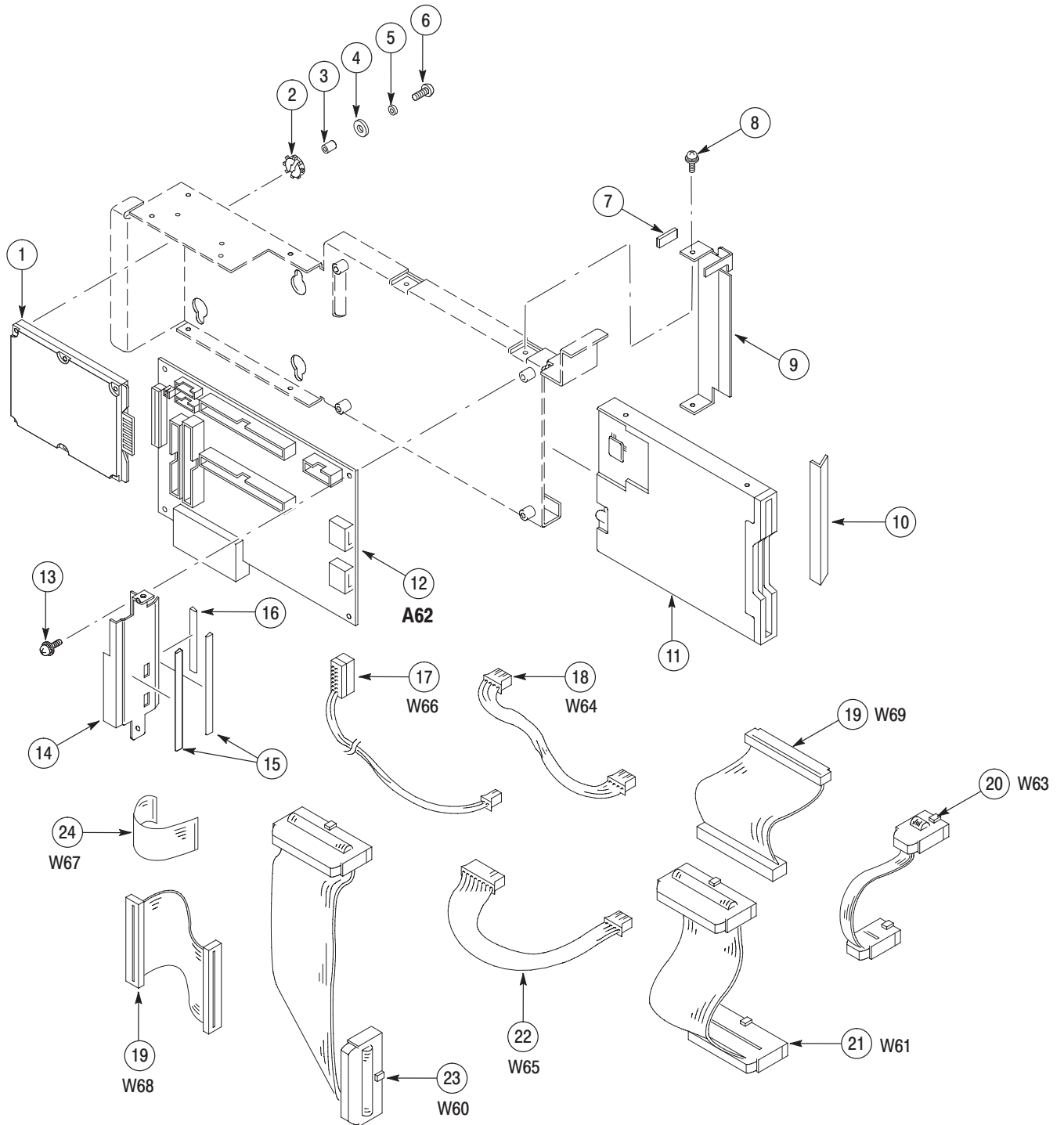
Figure 10-7: Disk modules
