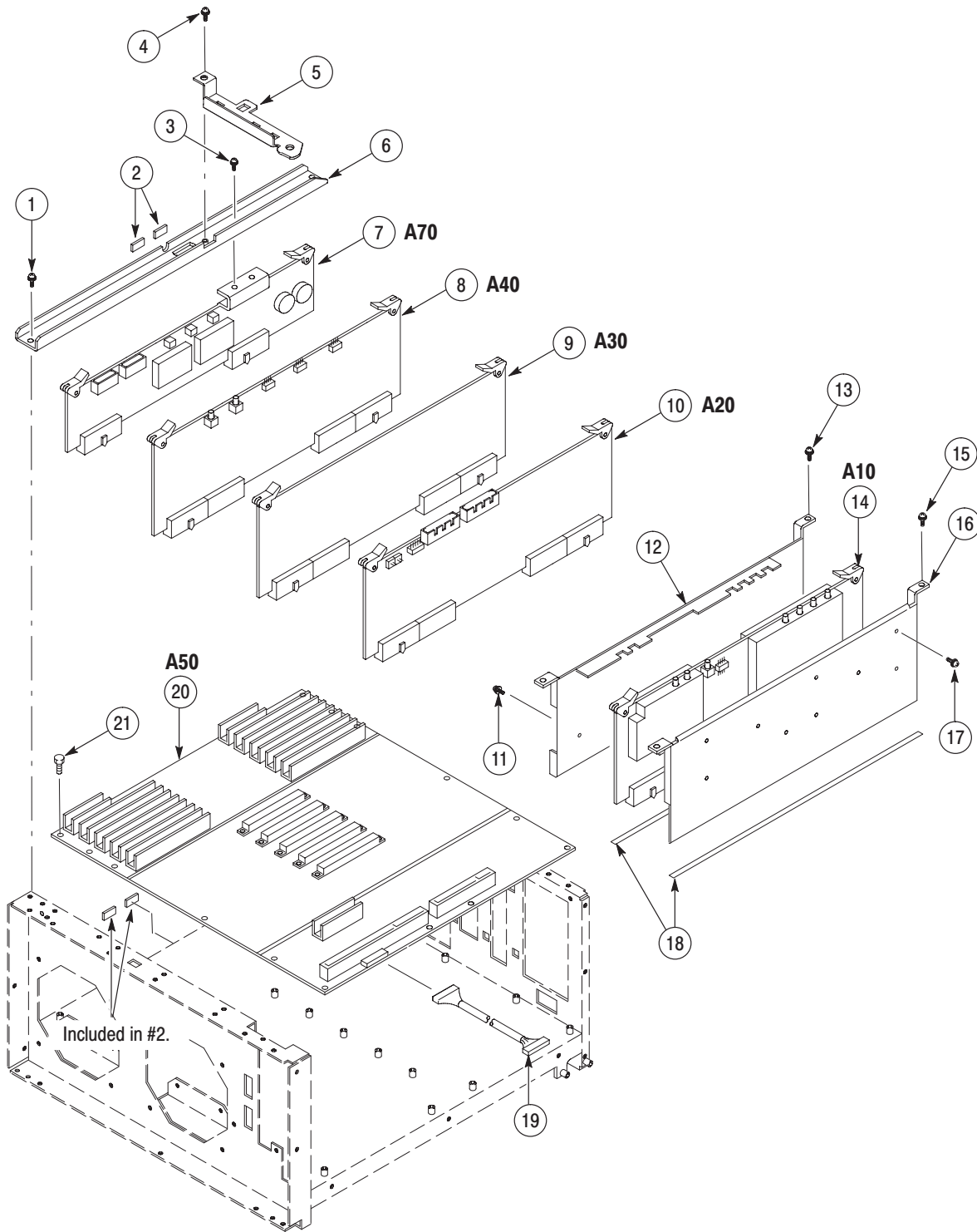
Figure 10-5: Mother board and its daughter boards - 1
