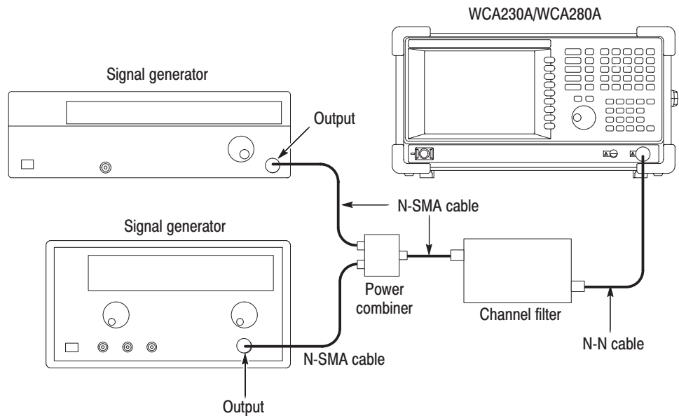
Figure 4-14: Initial test hookup
