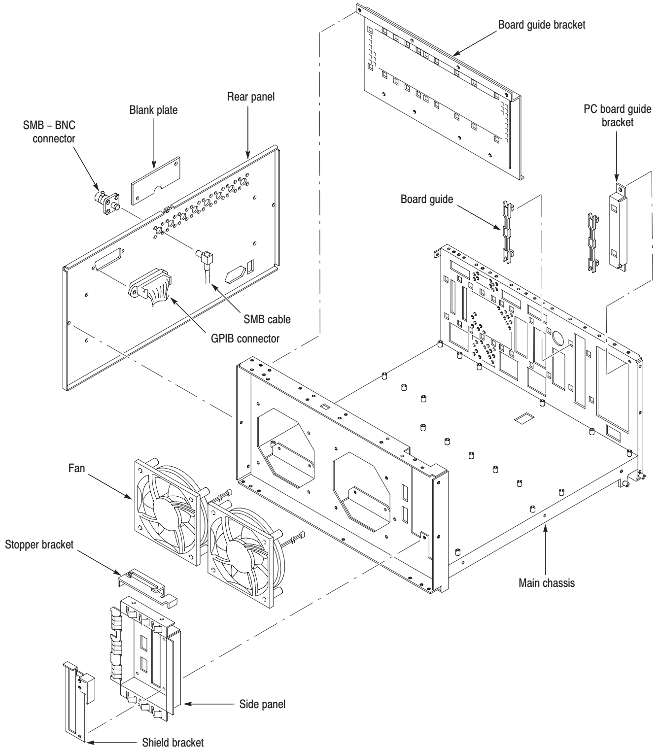
Figure 6-10: Chassis modules
