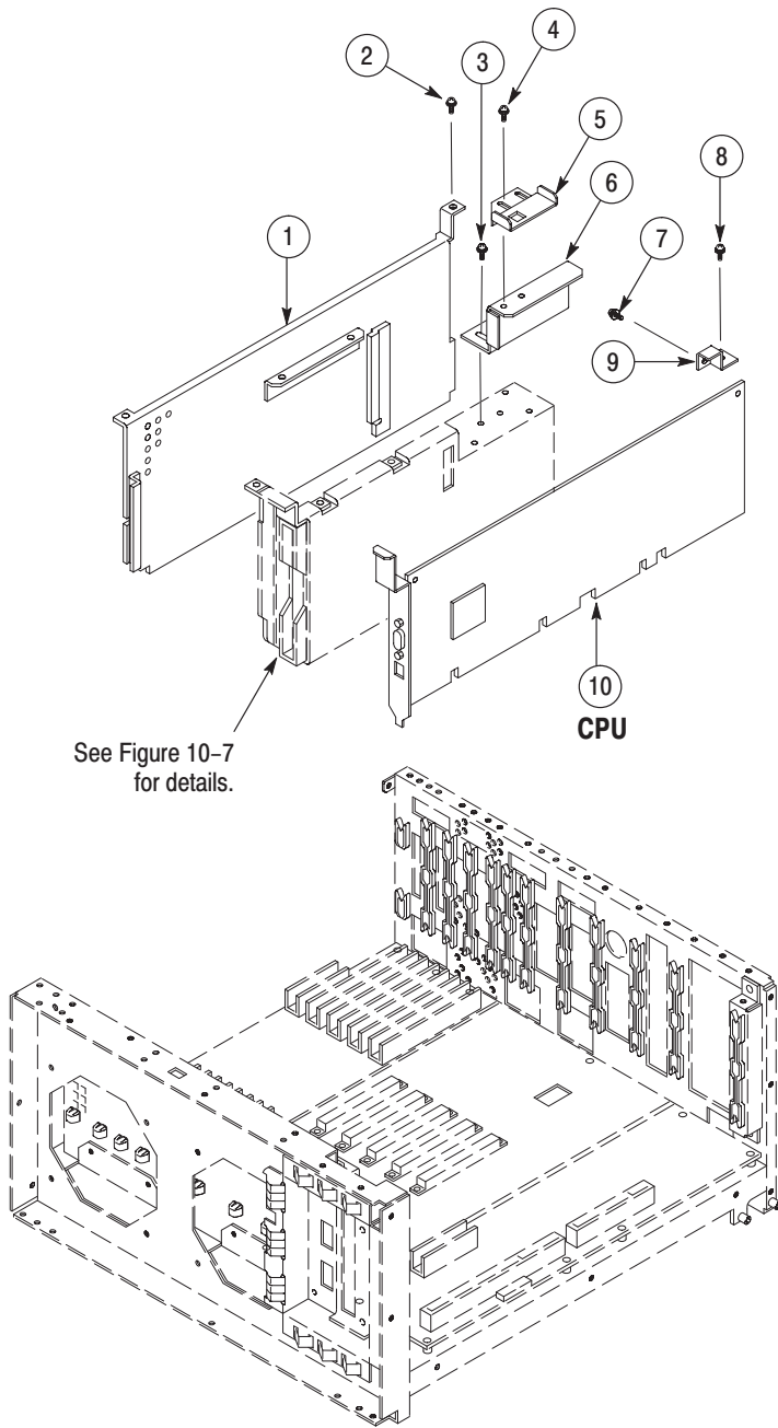
Figure 10-6: Mother board and its daughter boards – 2
