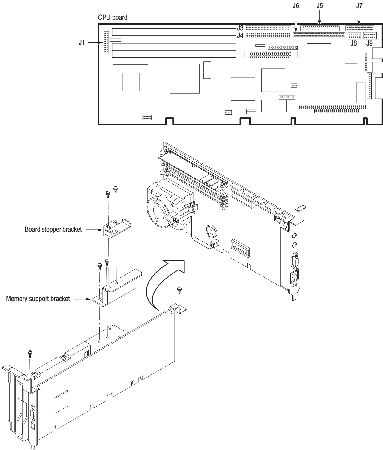
Figure 6-16: CPU board removal
