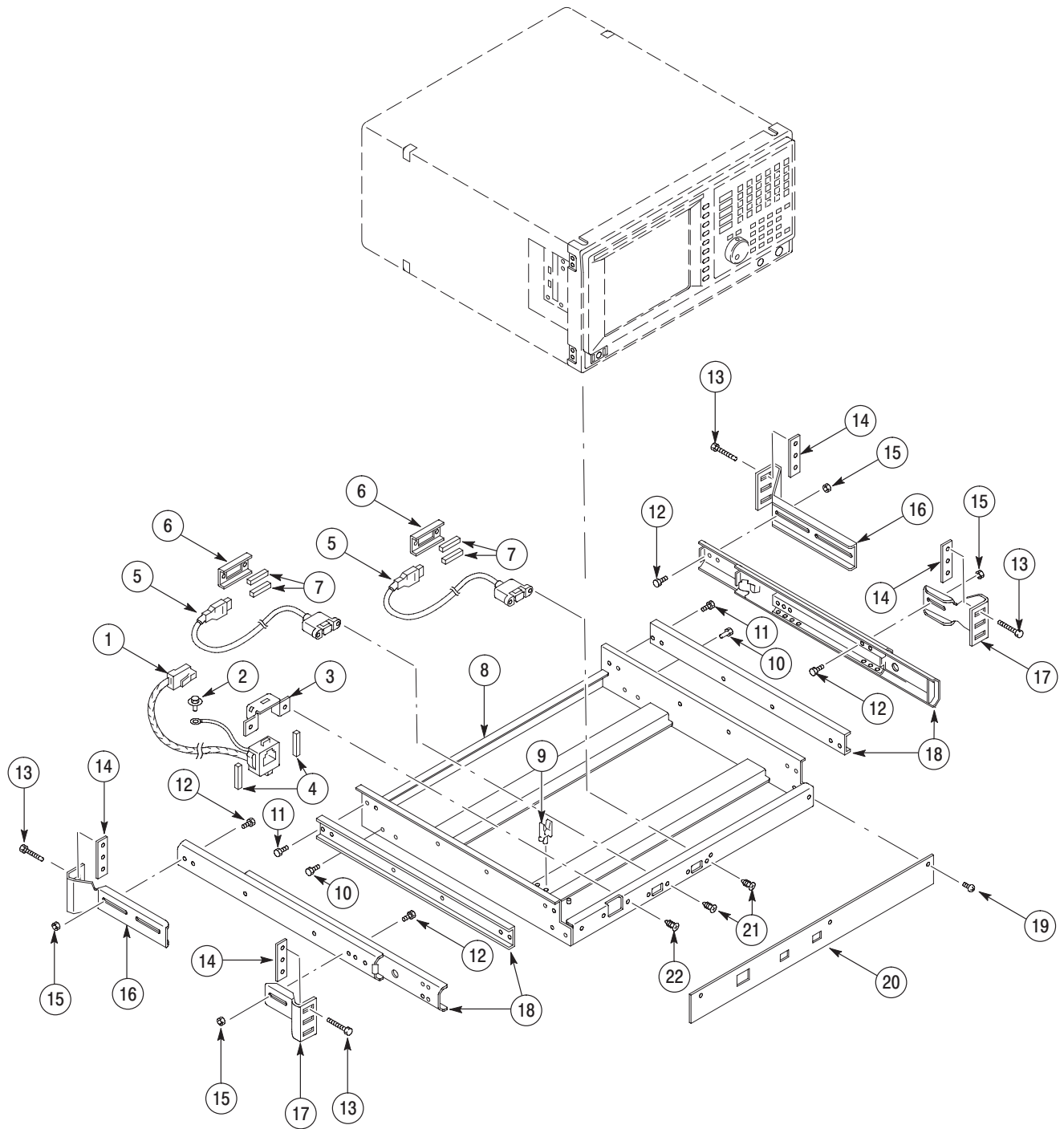
Figure 10-15: Rackmount - 2
